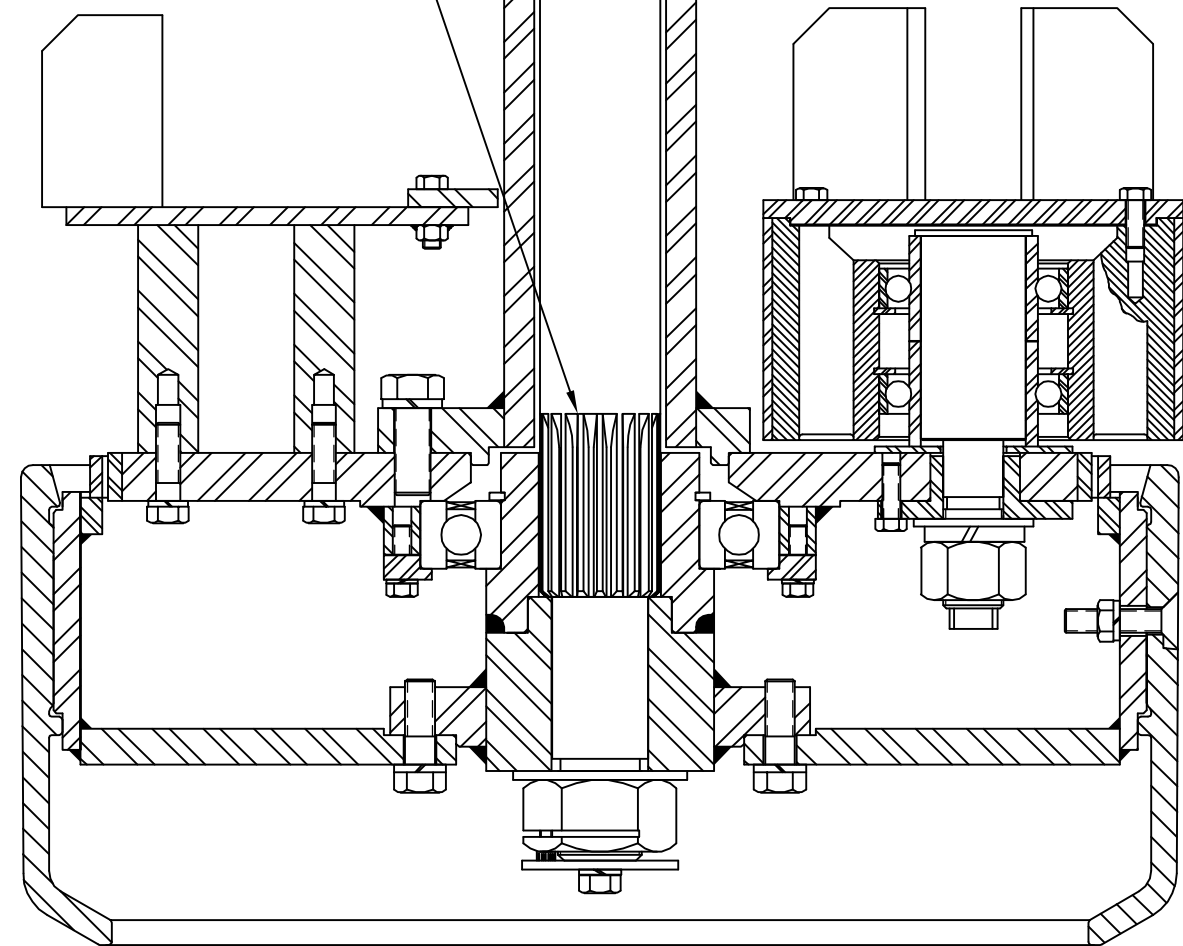
QUICKCHANGE SECTION VIEW
